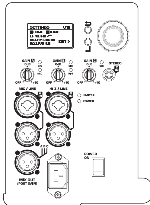
Back Panel
