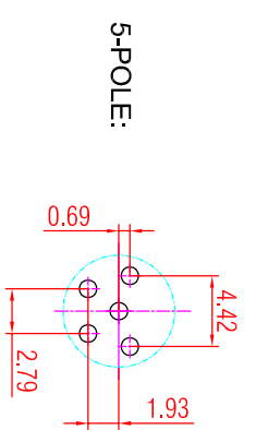
CONTACT LAYOUT
