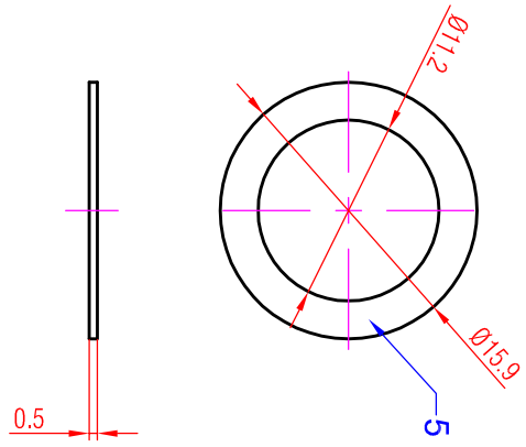
WASHER
