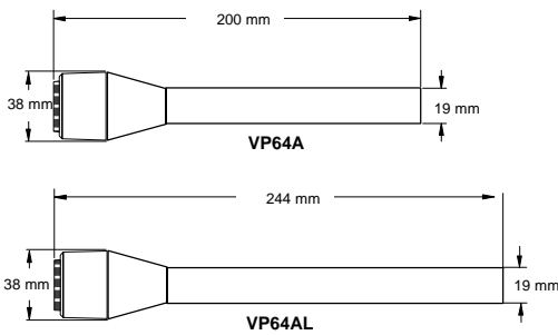
OVERALL DIMENSIONS
