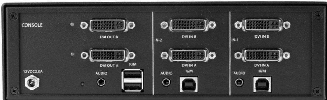
SDVN-2D Back
